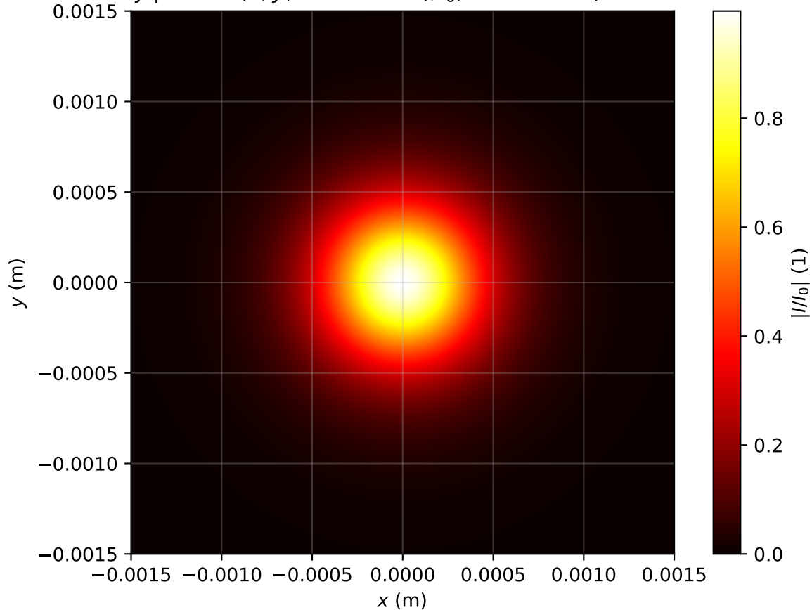
Intensity profile I(x, y, z = 3.423m)/I_0 , P_{in}=0.8P_{cr} , artificial time
